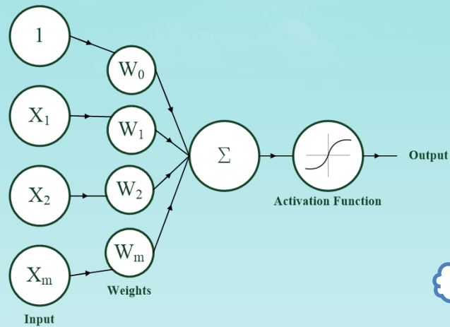
A single perceptron
